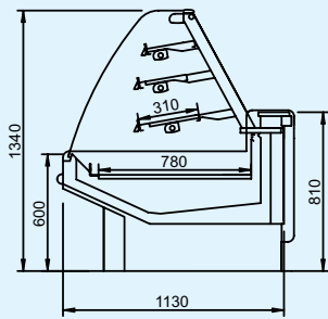
BA - 3 Shelf
